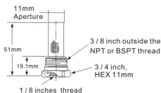
CY 38172 Type Adapter / strainer combination
